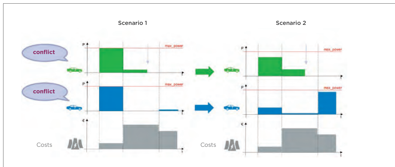
Figure 3. Practical example of load shifting
